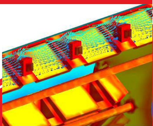
Aerothermics of a flow in an electric motor air-gap. (coll. Leroy-Somer) © PPRIME
